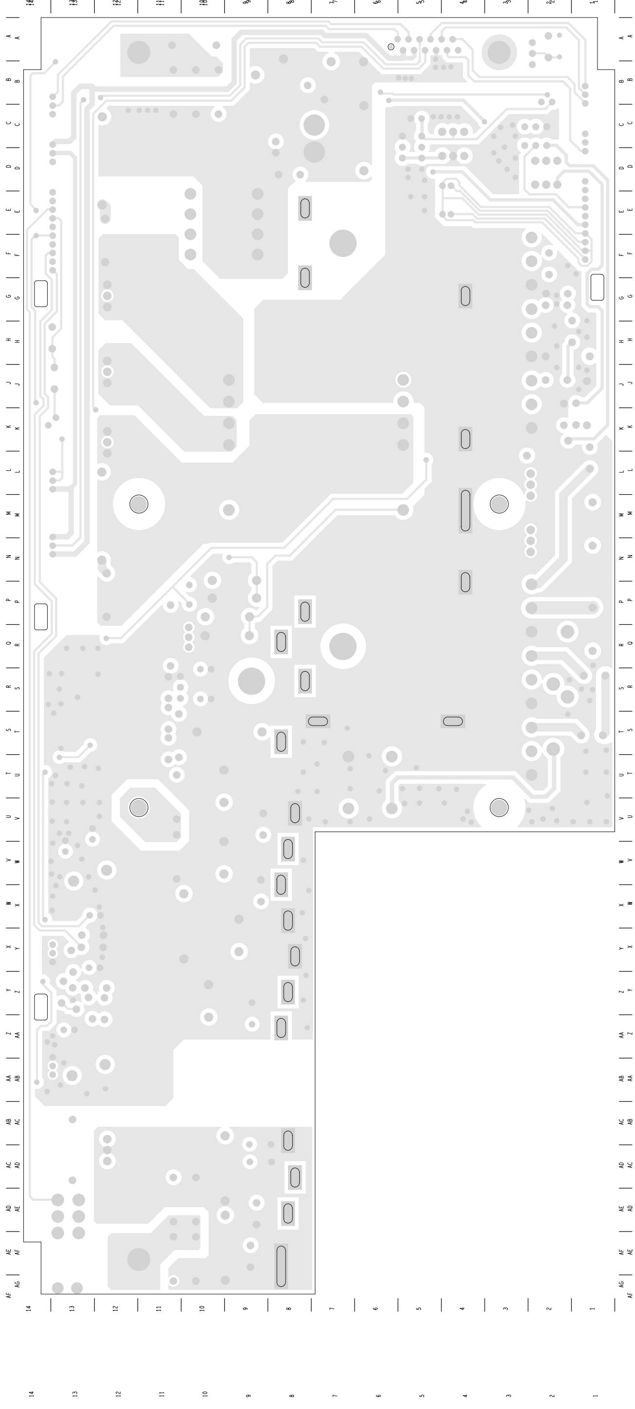
TAIT ELECTRONICS 226-02050-03 A 26Mar05 NTS TB8000 48V DC-DC CONVERTER LAYOUT-SECONDARY-SIDE
